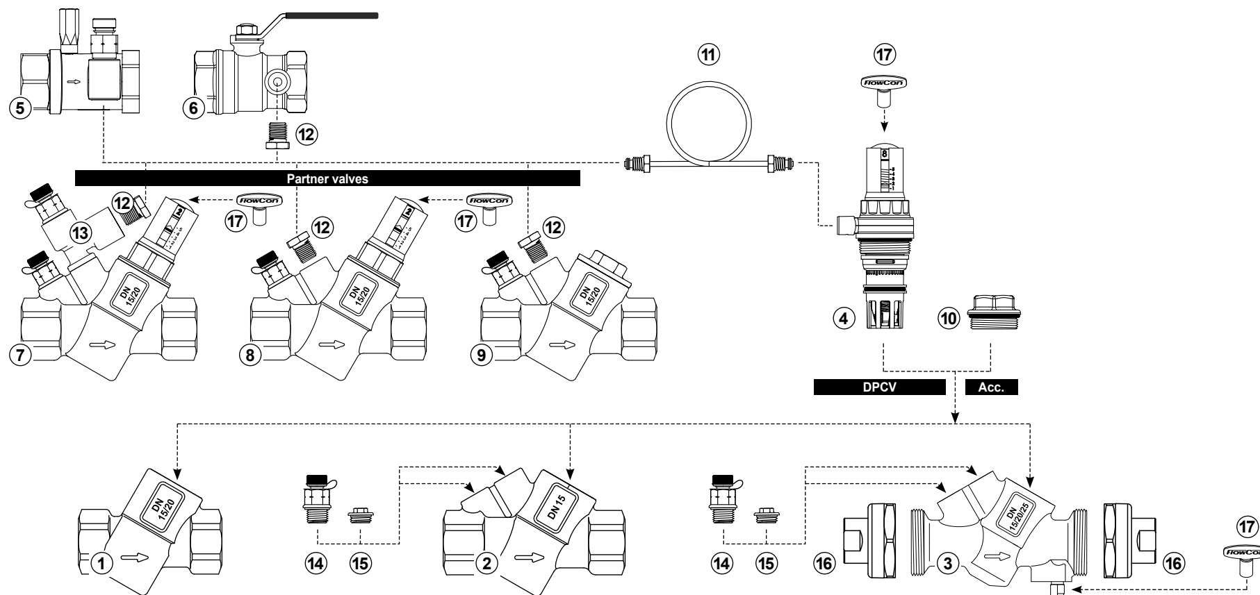
FlowCon EDR.1 DN15-25 (1/2"-1") • Differential Pressure Control Valve
